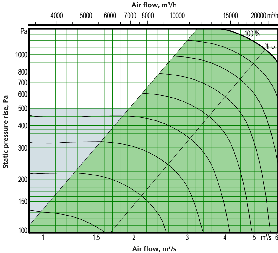
Motor shaft power: 10 kW (capacity variant 2)
